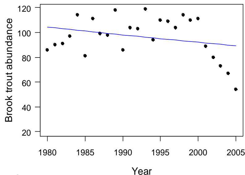
Figure APP 7.1. An example of a trend analysis where data in recent years do not fit the long term pattern.
