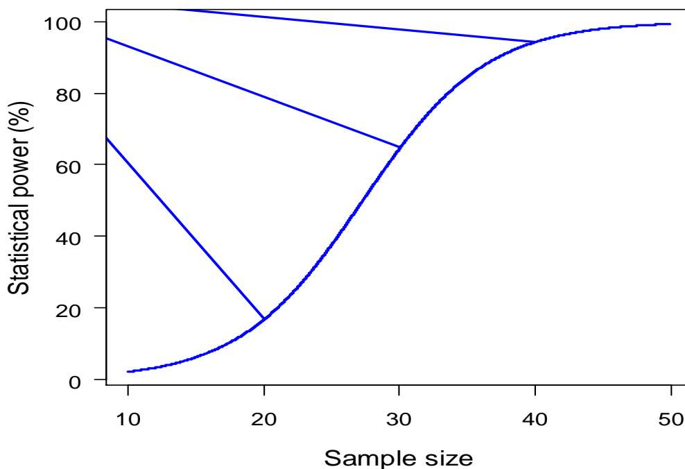
Figure APP 6.1. Example of a power curve. Note that the increase in power with sample size is not linear (all other factors held constant). In this example, taking more than 40 samples yields little gain in power
