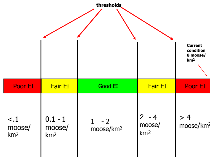
Figure APP 1.1: Thresholds for moose population density
